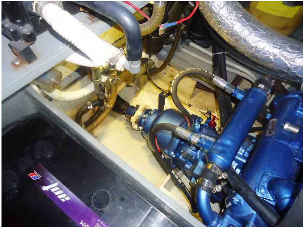
Borg-Warner reduction gear – note: new coupling
